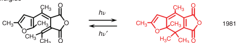
Diarylethene
