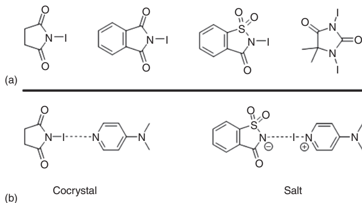
Figure 1.11 Representative examples of N -iodoimide halogen bond donors (a). Scheme of halogen bond cocrystal/salt concept transfer (b). ((b) Modified from Makhotkina et al. [105].)
