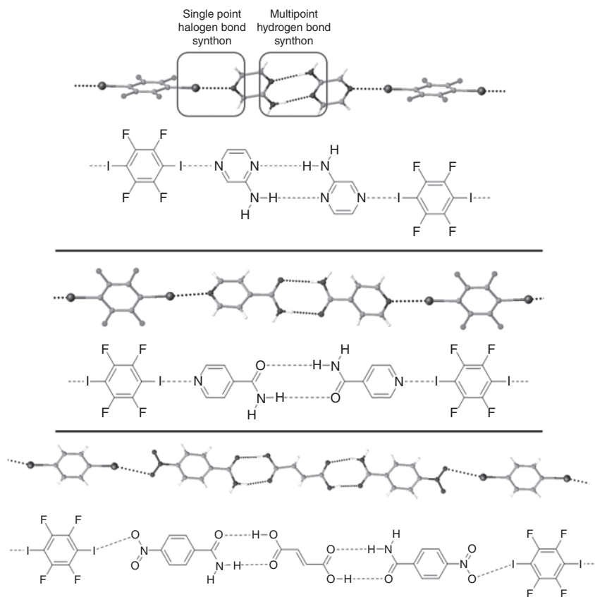
Figure 1.9 Examples of simultaneous halogen and hydrogen bonding in the construction of cocrystals. The top and middle figures highlights the single-point halogen bond synthon and the multipoint hydrogen bond synthon. The bottom structure is an example of a ternary cocrystal assembly utilizing hydrogen and halogen bond synthons. Dotted lines represent halogen or hydrogen bonds. CCDC Ref codes: PAMLIA (top). (Aakeröy et al. [78].) YIPCIK (middle). PILLIH (bottom). (Tothadi and Desiraju [79].)
