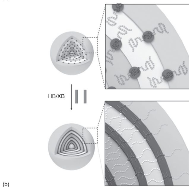
Figure 1.20 (a) Chemical structure of the halogen bond and hydrogen bond donors used in nanoparticle formation. (b) Tuning of the poly(4-vinylpyridine) (P4VP) volume with halogen bond and hydrogen bond donors and transition from lamella-sphere to lamella-lamella morphology. Source: From Quintieri et al. [186]. © 2018 MDPI.
