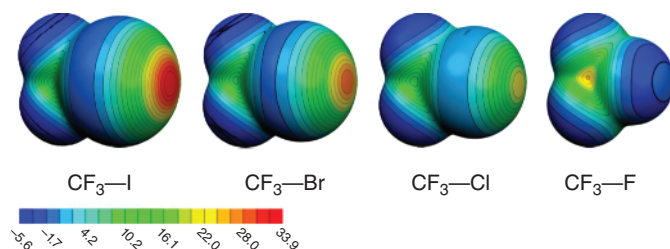
Figure 1.2 Molecular electrostatic potential maps drawn at the isodensity surface of 0.001 au for \text{CF}_3\text{I} , \text{CF}_3\text{Br} , \text{CF}_3\text{Cl} , and \text{CF}_4 . All maps are drawn at the same scale, and values are in kcal/mol. Source: From Clark et al. [8]. © 2007 Springer Nature.
