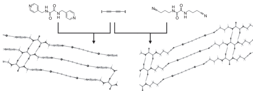
Figure 1.13 Cocrystallization components and pre-polymerization structures of 1,4-diiodo-1,3-butadiene with oxalamide derivatives. CCDC ref codes: WANNUV01 (left), CEKFUU (right).
