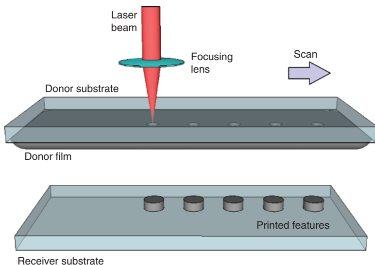
Figure 1.1 Principle of operation of the LIFT technique.
