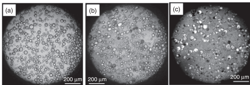
Figure 1.9 Observation of freeze-drying an oil-in-water emulsion (cyclohexane emulsified into aqueous PVA solution) using an optical microscope. (a) The emulsion as prepared, spread on a glass slide; (b) this emulsion is frozen in the freezing stage; and (c) the same sample after freeze-drying by subjecting the freezing stage compartment to a vacuum pump.
