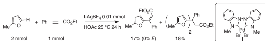
Figure 1.8 Hydroarylation of ethyl phenylpropiolate using a dicarbene Pd(II) complex.
