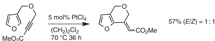
Figure 1.13 Intramolecular hydroarylation of a furan-yne substrate.
