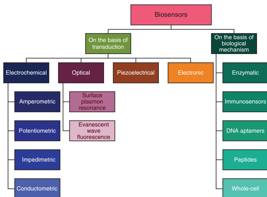
Figure 1.5 Biosensors classification.
