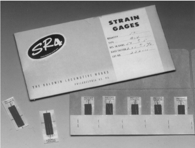
Fig. 1.5 One of the first strain gage packages as sold by Baldwin in 1941
