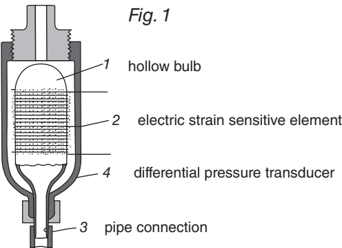
Fig. 1.6 ‘Bonded strain gage pressure transducer’, resistance wire wound on a thin-walled tube with closed ends [1.11]
