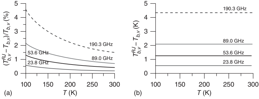
Figure 1.2 (a) Relative and (b) absolute variations of the brightness temperature with black-body temperature varying from 100 to 300 K at frequencies 23.8, 53.6, 89.0, and 190.3 GHz. (Weng and Zou 2013 [2]. Reproduced with permission of Optical Society of America.)
