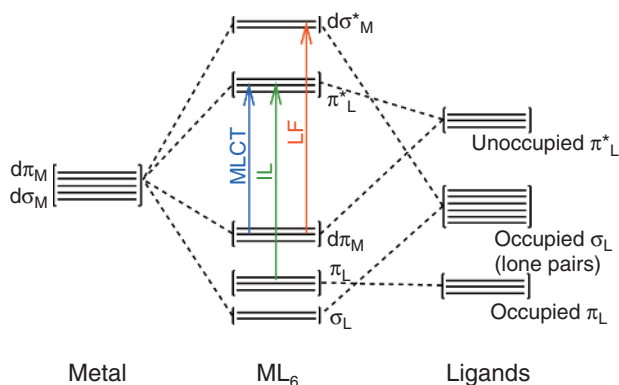
Scheme 1.3 Simplified molecular orbital diagram for an octahedral compound with \pi -acceptor ligands. The three types of electronic transitions discussed in the text are indicated by the arrows.
