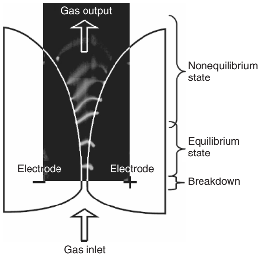
Figure 1.10 Nice example of the superposition of several short exposures of the different stages of a gliding arc discharge. The extension of the discharge channel is clearly visible in the nonthermal stage (upper part). (Source: Taken with permission from Fridman [29].)
