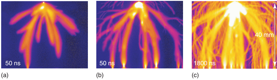
Figure 1.4 Streamer discharges in a 40 mm gap in atmospheric air with a 54 kV pulse, 30 ns risetime, and half-width of about 70 ns. The images are acquired with short (a,b) and long (c) exposure times.
