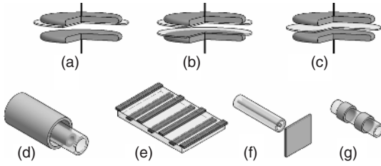
Figure 1.7 Dielectric barrier discharge configurations: (a–c) plane barriers, mostly used in research, (d) coaxial design, often used in ozonizers, (e) (partly) buried electrodes for surface discharge, and (f,g) plasma jets as used in, for example, biomedical applications.
