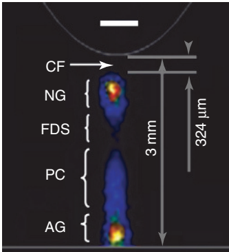
Figure 1.5 Example of an atmospheric pressure air glow discharge in a metal pin (top) water electrode (bottom) geometry. The typical structures of the low-pressure glow discharge are clearly visible, although on a sub-millimeter scale. (CF) cathode fall; (NG) negative glow; (FDS) Faraday dark space; (PC) positive column; (AG) anode glow. (Source: Taken with permission from Ref. [20].)
