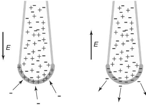
Figure 1.3 Illustration of downward propagating positive (a) and negative (b) streamers. The plus symbols indicate positive ions, while the minus symbols indicate negative ions or free electrons.
