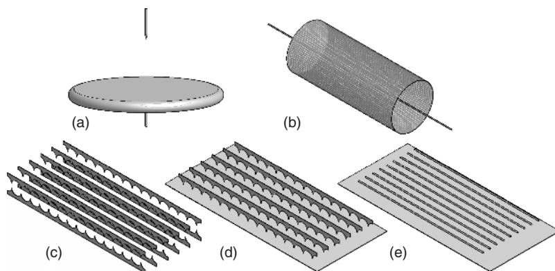
Figure 1.1 Schematic depictions of popular electrode geometries in corona reactors: (a) point-plane, (b) wire-cylinder, (c) double sawblade, (d) sawblade-plane, and (e) wire-plane. The high voltage is applied to the following parts: (a) top needle, (b) central wire, and (c–e) top sawblade/wires. The other parts are grounded.
