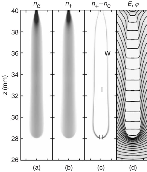
Figure 1.2 Structure of positive streamers shown by zooming into the relevant region of a simulation by Ratushnaya et al. The panels show (a) electron density n_e , (b) ion density n_+ , (c) space charge density ( n_+ - n_e ), as well as (d) electric field strength E and equipotential lines \varphi . The letters in (c) indicate the streamer regions: H – streamer head, I – interior, and W – wall of the streamer channel. (Source: Image from Ref. [71].)
