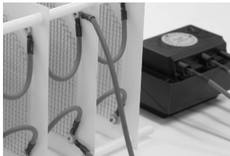
Figure 1.8 PlasmaNorm® demonstration unit, that is, a dielectric barrier discharge made from plastic sheets with a metal mesh on both sides. The power supply is a 50 Hz high-voltage transformer. (Source: Courtesy of Circlair Benelux BV.)
