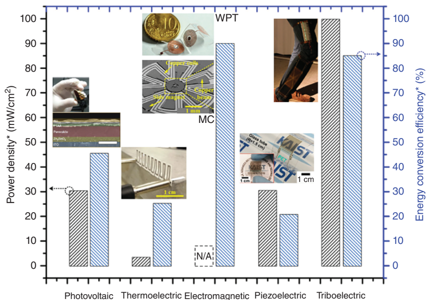
Figure 1.2 Summary of technical progress of five promising methods for harvesting energy from the environment. Source: Reproduced with permission from Zhang et al. [4]. Copyright 2018, Elsevier.
