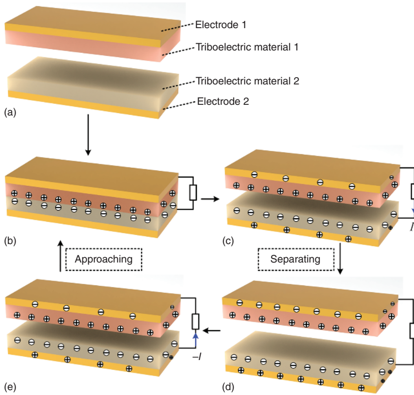
Figure 1.3 The working principle of contact-separation-mode triboelectric nanogenerators (TENGs). (a) In the beginning, the triboelectric pair made of triboelectric materials 1 and 2 are separated, and the whole device shows an electrically neutral state. (b) When a compressive force is applied, the top structures will move toward the bottom structures and have a friction with each other. Due to the phenomenon of triboelectrification effect, positive and negative charges of equal amount will be generated on the surfaces of triboelectric pair, respectively. (b–d) When the compressive force is removed, the triboelectric pair will separate from each other as a result of the mechanical recovery force. And then, an internal electric potential is established, which changes accordingly as the distance of the triboelectric pair increases and decreases. Consequently, due to the electrostatic induction, opposite charges are generated on the back electrodes, and a current ( I ) can be detected in the loop resulting from the charges flowing from one electrode to the other. When the triboelectric pair works cyclically, an electric output power will be generated continuously. Source: Reproduced with permission from Zhang et al. [4]. Copyright 2018, Elsevier.
