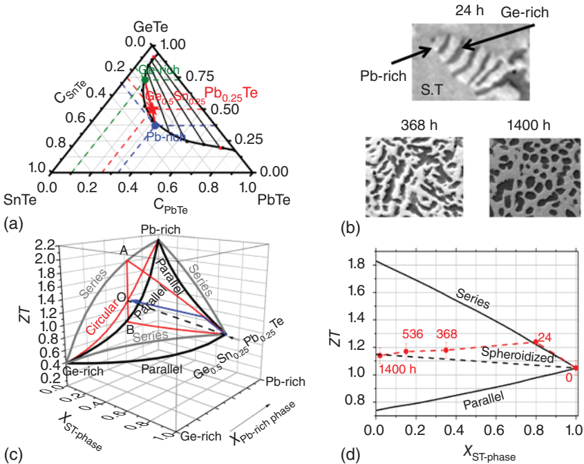
Figure 1.5 Quasi-ternary GeTe—PbTe—SnTe phase diagram showing a well-defined miscibility gap (a), as well as morphological (b), 3-D ZT (c), and 2-D ZT (d) variations upon thermal treatment at 400 °C for different durations for the p-type Ge 0.5 Pb 0.25 Sn 0.25 Te composition. (Gelbstein 2012 [4]. Reproduced with permission of Elsevier.)
