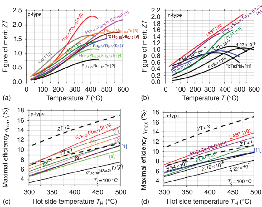
Figure 1.1 ZT values of the most efficient IV–VI alloys recently published – the p-type: \text{Pb}_{0.98}\text{Te} [1], \text{Pb}_{0.99}\text{Na}_{0.01}\text{Te} [2], \text{Ge}_{0.87}\text{Pb}_{0.13}\text{Te} [3], \text{Ge}_{0.5}\text{Pb}_{0.25}\text{Sn}_{0.25}\text{Te} [4], \text{Pb}_{0.96}\text{Sr}_{0.04}\text{Te} (2%Na) [5], \text{Ag}_{0.9}\text{Pb}_{0.5}\text{Sn}_{0.3}\text{Sb}_{0.7}\text{Te}_{10} – LASTT [6], \text{Na}_{0.95}\text{Pb}_{20}\text{SbTe}_{22} – SALT [7], \text{Pb}_{0.97}\text{Mg}_{0.03}\text{Te} :Na [8], \text{PbTe}_{0.85}\text{Se}_{0.15} :2%Na [9]; and n-type: \text{AgPb}_{18}\text{SbTe}_{20} – LAST [10], \text{PbTe} (0.1 at%In) [11], \text{PbI}_2 doped \text{PbTe} with various carrier concentrations of 6.54 \times 10^{18} , 2.19 \times 10^{19} , 4.22 \times 10^{19} and 6.09 \times 10^{19}/\text{cm}^3 [11], \text{K}_{0.95}\text{Pb}_{20}\text{Sb}_{1.2}\text{Te}_{22} – PLAT [12], and (\text{Pb}_{0.95}\text{Sn}_{0.05}\text{Te})_{0.92}(\text{PbS})_{0.08} :0.055 mol% \text{PbI}_2 [13]. (Pei et al. 2012 [8]. Reproduced with permission of Nature Publishing Group.)
