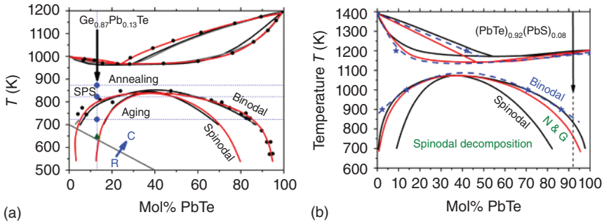
Figure 1.4 Quasi-binary PbTe—GeTe (a) [3] and PbTe—PbS (black curve [27], red curve [28], and blue curve – calculated for 100% Pb 0.95 Sn 0.05 Te instead of PbTe based on the PbTe—SnTe phase diagram [27]) and (b) phase diagrams showing a miscibility gap and a tendency for phase separation. The highly efficient (Pb 0.95 Sn 0.05 Te) 0.92 (PbS) 0.08 and Ge 0.87 Pb 0.13 Te thermoelectric compositions are clearly indicated. For the PbTe—GeTe phase diagram the transition temperatures from rhombohedral (R) to cubic (C) structures are also indicated. (Volykhov et al. 2006 [27]. Reproduced with permission of Springer.)
