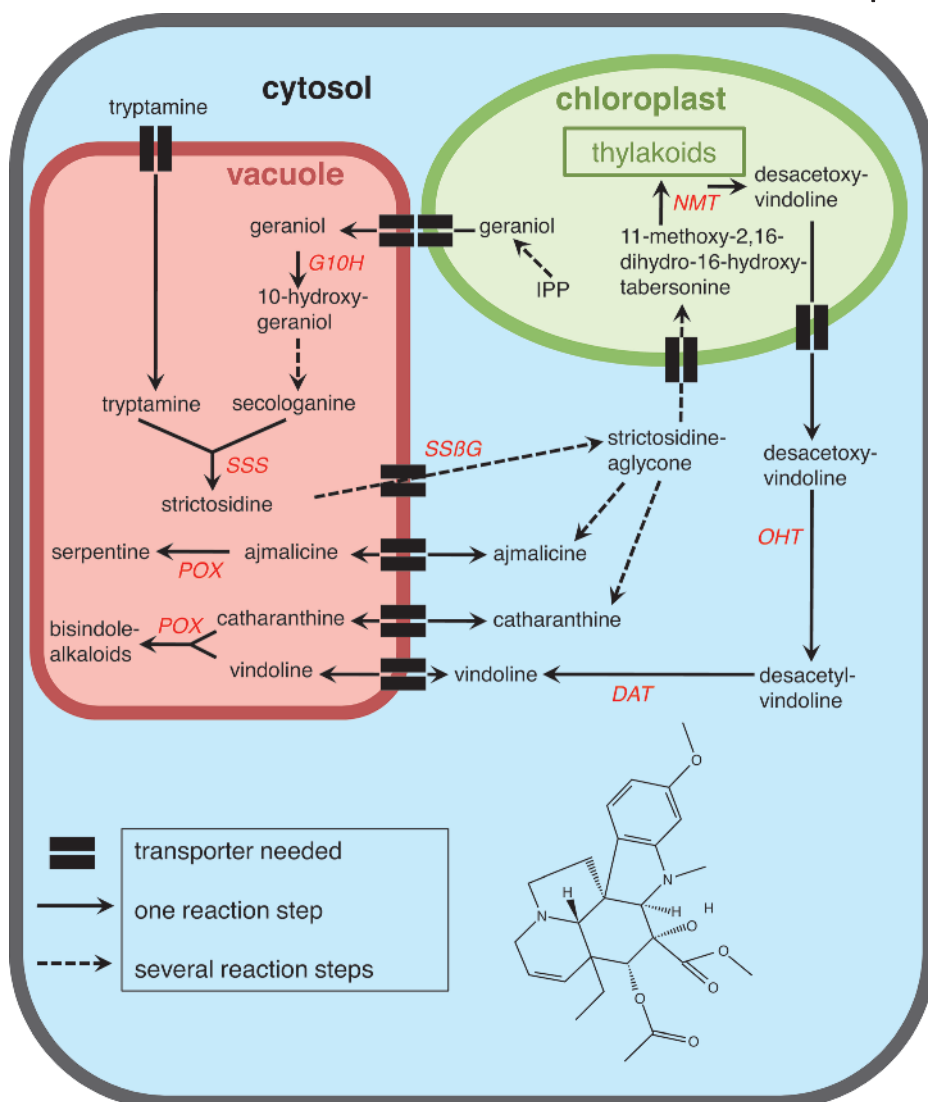
Figure 1.6 Compartmentation of terpene indole alkaloid biosynthesis in Catharanthus roseus . The cellular compartments (plastids, cytosol and vacuole) participate in the biosynthetic steps. Enzymatic reactions with dashed arrows are hypothetical. Circles symbolize membrane-associated enzymes. Putative transporters are also indicated. The structure for the terpene indole alkaloid vindoline is shown. IPP: isopentenylpyrophosphate; G10H: geraniol-10-hydroxylase; NMT: S-adenosyl-
