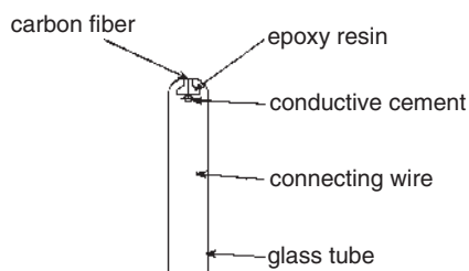
Figure 1.1 Cross section of a simple microelectrode.
