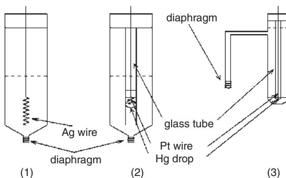
Figure 1.2 Cross sections of various types of reference electrodes. (1): Silver/silver chloride electrodes. (2 and 3): Calomel or mercurous sulfate electrode. Dotted lines indicate solution filling level.
