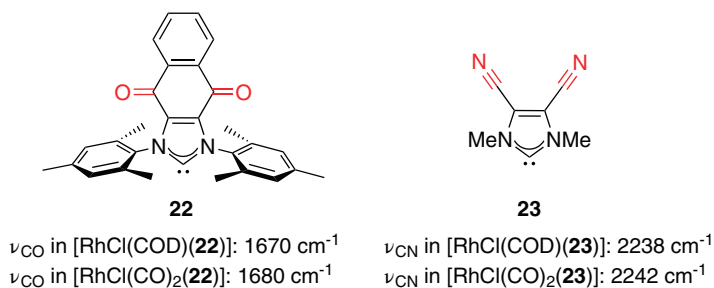
Figure 1.14 Spectroscopic investigation of \pi -backbonding in [\text{RhCl}(\text{COD})(\text{NHC})] and [\text{RhCl}(\text{CO})_2(\text{NHC})] complexes.
