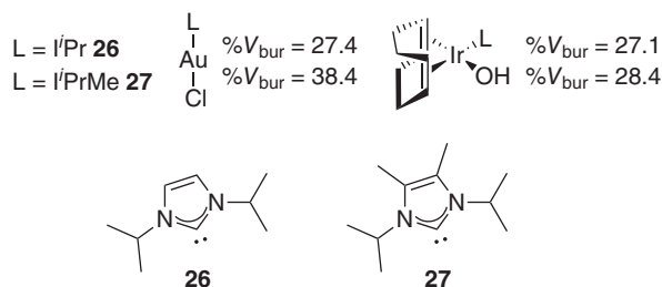
Figure 1.18 Comparison of \%V_{\text{bur}} using different metal complexes.
