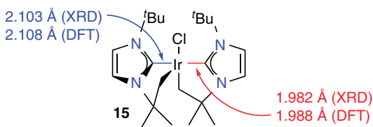
Figure 1.10 Ir–C bond lengths in [\text{IrCl}(\text{I}^t\text{Bu})_2] [31].
