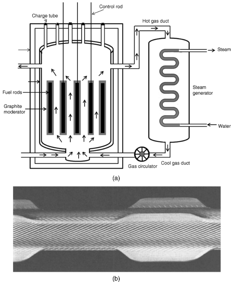
Figure 1.8 (a) A schematic of a Magnox reactor. (b) A part of the magnesium alloy fuel can of a British Magnox reactor. Courtesy: Light Alloys by Ian Polmear.
