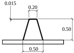
Figure 1.16 – Detailed view of longitudinal stiffener
