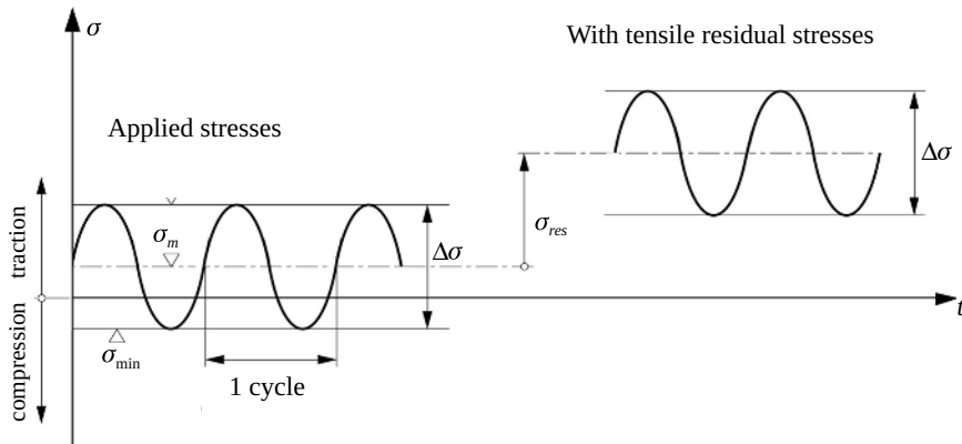
Figure 1.2 – Definition of stresses and influence of tensile residual stresses (TGC 10, 2006)
