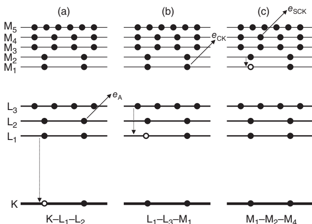
Figure 1.4 Schematic illustration of the non-radiative transitions Auger (a), Coster-Kronig (b), and Super Coster-Kronig (c). In an Auger transition, an electron e_A is ejected from a higher shell; the transition shown is K-L 1 -L 2 . In a Coster-Kronig transition, a vacancy in any subshell is filled by an electron in a higher subshell in the same shell, with the ejection of an electron e_{CK} from a higher shell (L 1 -L 3 -M 1 shown). In a Super Coster-Kronig transition, the electron e_{SCK} is ejected from the same shell (M 1 -M 2 -M 4 shown).
