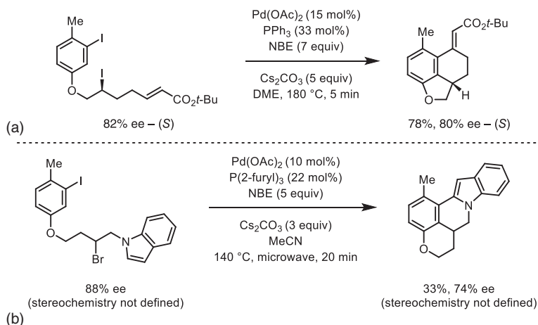
Scheme 1.40 Study on the erosion of enantiomeric excess using enantioenriched substrates in (a) DME and (b) MeCN as solvents.
