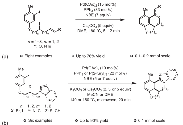
Scheme 1.39 Intramolecular ortho -alkylation followed by intramolecular (a) ipso -Heck termination (b) ipso C–H arylation.
