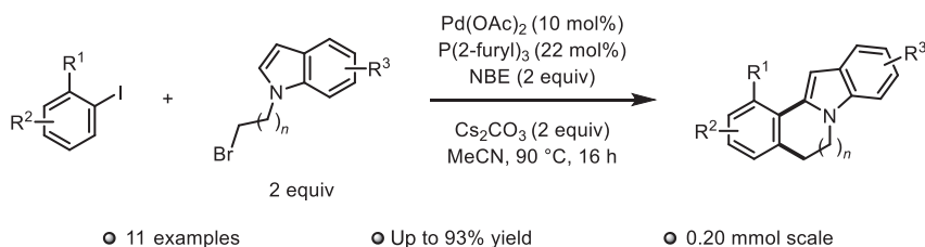
Scheme 1.8 Synthesis of annulated indoles via ipso C–H arylation.
