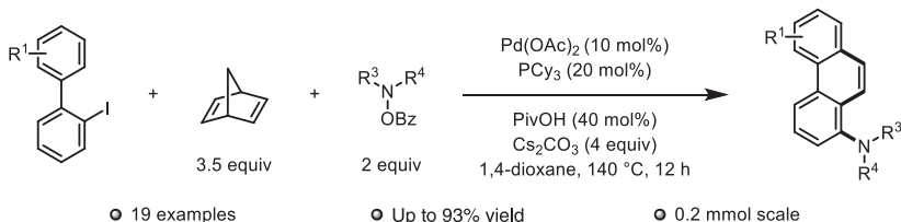
Scheme 1.57 Synthesis of aminated phenanthrenes.
