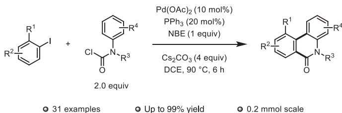
Scheme 1.26 First use of carbamoyl chlorides in Pd/NBE chemistry.
