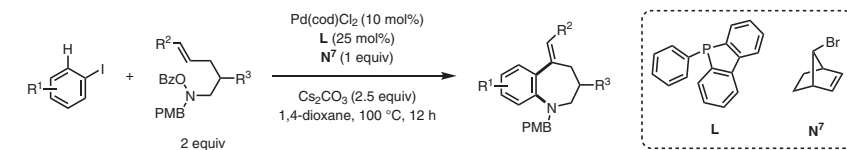
Scheme 1.29 Synthesis of C3,C4-disubstituted indoles via ortho -amination/ ipso -Heck termination.
