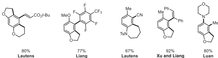
Scheme 1.38 Subsequent examples of intramolecular ortho -functionalization followed by intermolecular ipso -termination.
