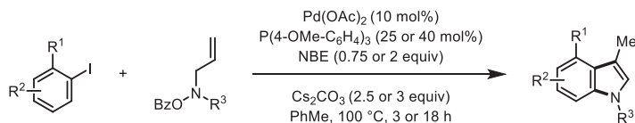
Scheme 1.29 Synthesis of C3,C4-disubstituted indoles via ortho -amination/ ipso -Heck termination.
