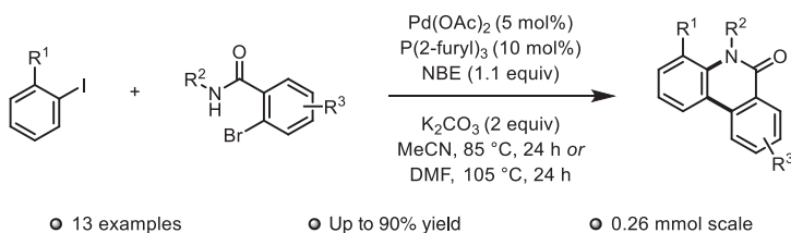
Scheme 1.17 Synthesis of 6-phenanthridinones.
