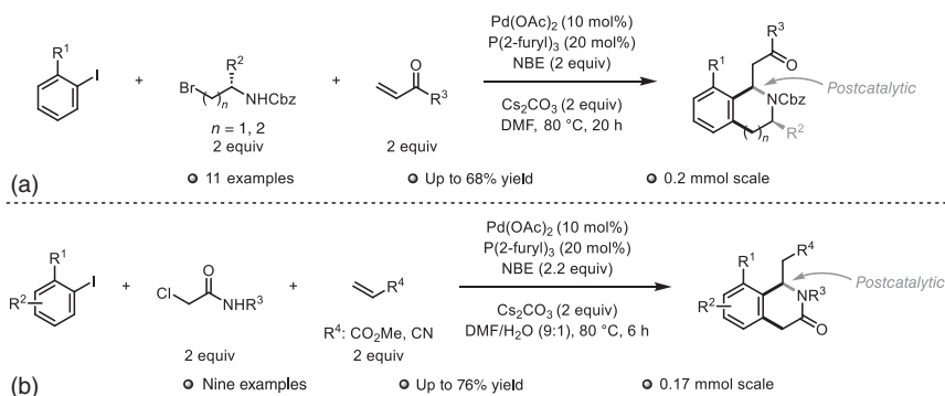
Scheme 1.59 Synthesis of N-heterocycles via a postcatalytic aza-Michael addition using activated alkenes and (a) N-Cbz-bromoalkylamines (b) \alpha -chloroamides.
