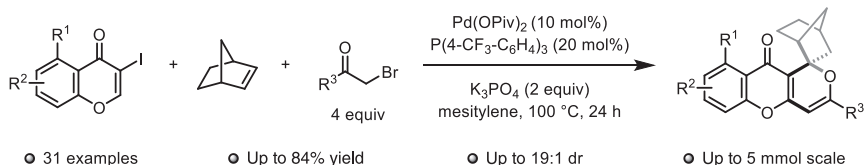
Scheme 1.63 Postcatalytic intramolecular Michael addition onto an NBE moiety.
