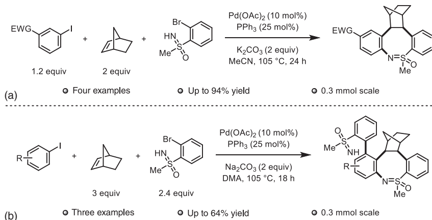
Scheme 1.51 Synthesis of NBE- and sulfoximine-containing adducts using (a) one equivalent of 2-bromo-NH-sulfoximine (b) two equivalents of 2-bromo-NH-sulfoximine.
