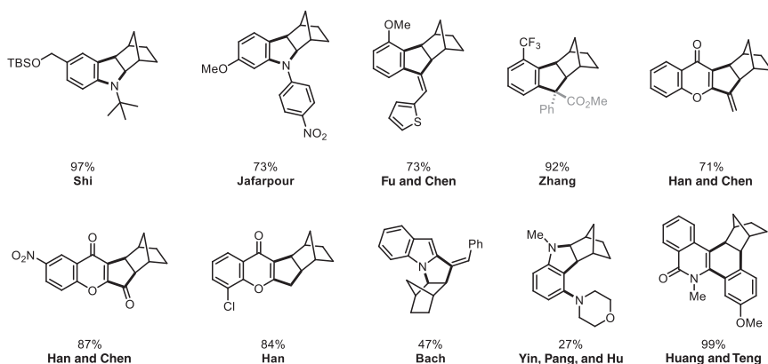
Scheme 1.52 Subsequent examples of NBE-containing adducts.
