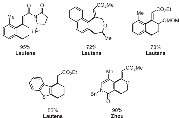
Scheme 1.4 Examples of ortho -alkylation/ ipso -Heck-termination annulative methodologies.
