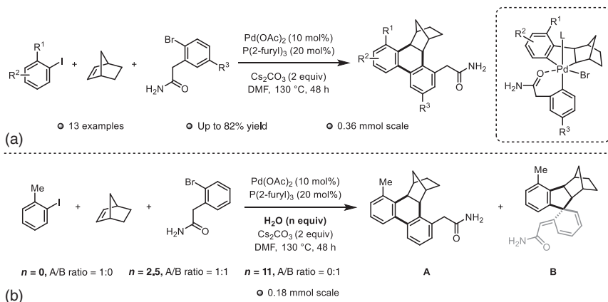
Scheme 1.49 Synthesis of NBE-containing adducts due to a coordinating amide-moiety (a) general reaction conditions (b) study of the effect of added water on the selectivity of the reaction.
