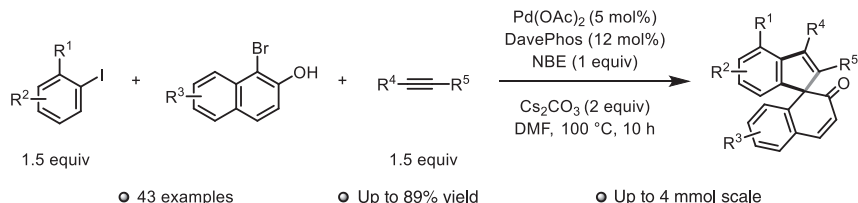
Scheme 1.42 Synthesis of triphenylenes from an aryl iodide and two ortho -bromoarylcarboxylic acids.
