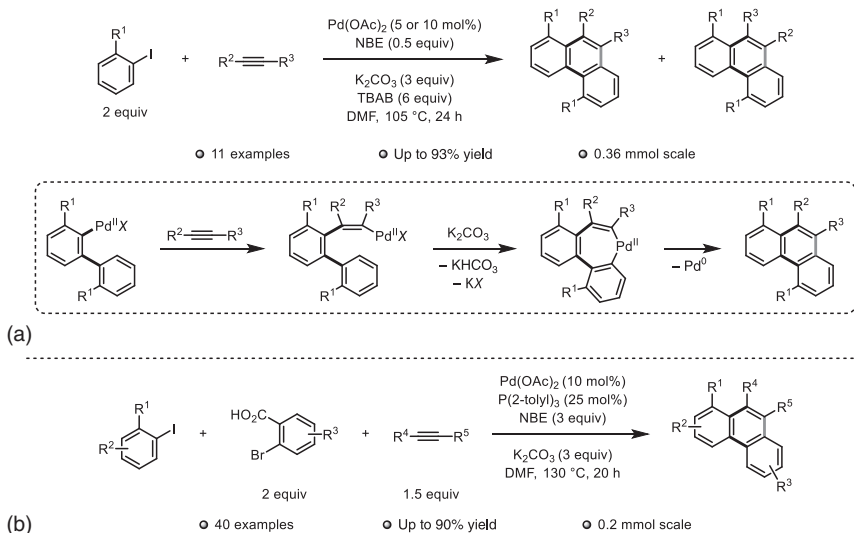
Scheme 1.41 Synthesis of phenanthrenes from an alkyne and (a) two identical aryl iodides (b) two different aryl halides.
