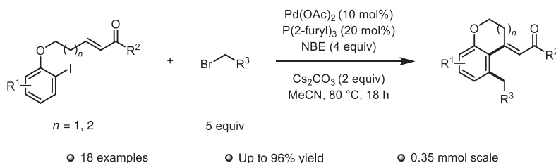
Scheme 1.34 First methodology of ortho -functionalization with an external reagent followed by intramolecular ipso -termination.
