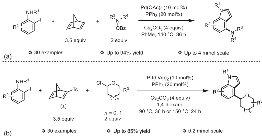
Scheme 1.56 Synthesis of C4-functionalized indoles via (a) ortho -amination (b) ortho -glycosylation.
