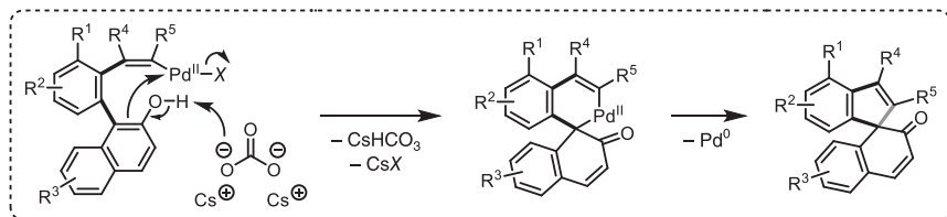
Scheme 1.43 Synthesis of spirocarbocycles from aryl iodides, bromonaphthols, and alkynes.
