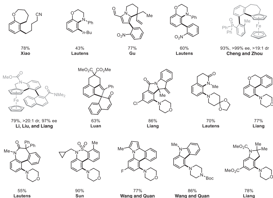
Scheme 1.35 Subsequent examples of ortho -functionalization with an external reagent followed by intramolecular ipso -termination.
