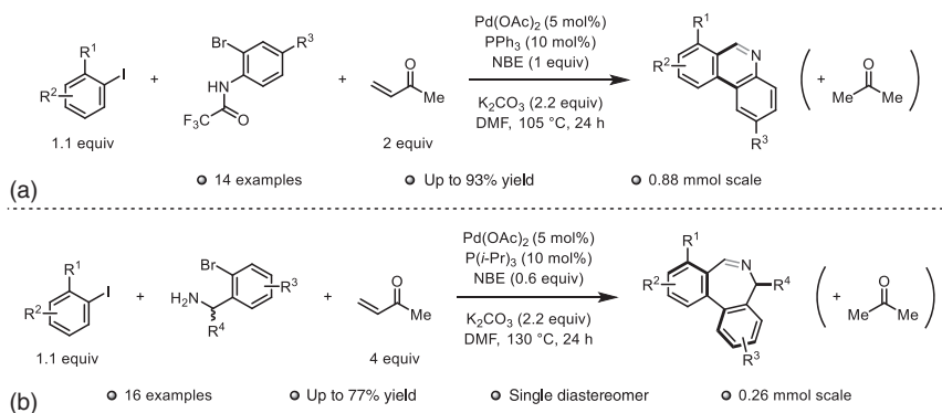
Scheme 1.62 Postcatalytic retro-Mannich reactions using MVK as the ipso -terminating reagent to form (a) phenanthridines and (b) imines.
