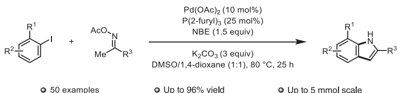
Scheme 1.32 Indole formation via reversal of traditional regioselectivity of the electrophilic and terminating groups.
