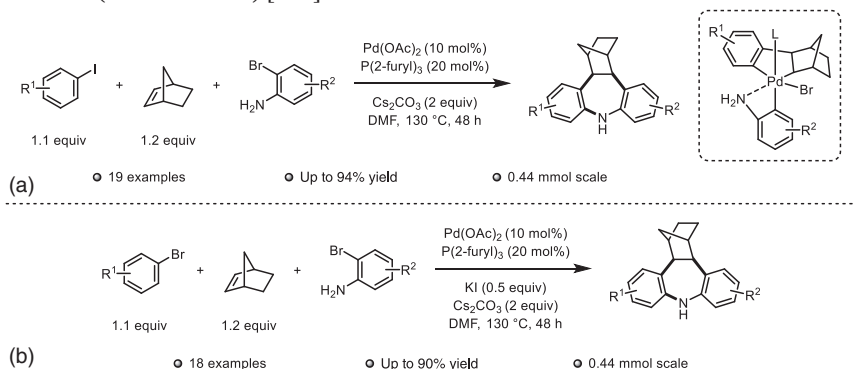
Scheme 1.50 Synthesis of NBE-containing azacycles following C(sp^2)-C(sp^3) reductive elimination using (a) aryl iodides (b) aryl bromides.
