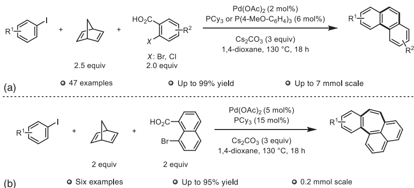
Scheme 1.58 Synthesis of (a) phenanthrene derivatives and (b) heptagon-embedded aromatic compounds via ortho -arylation.
