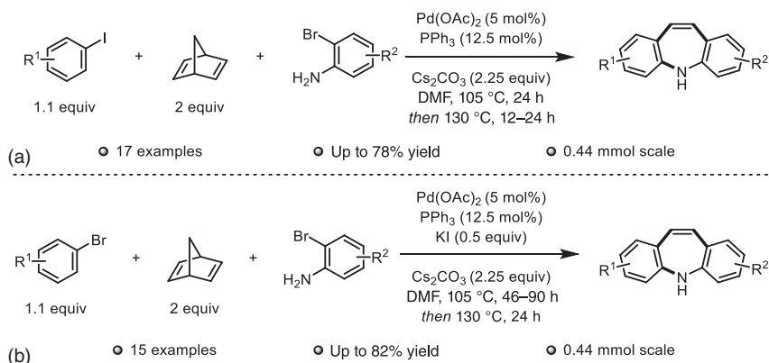
Scheme 1.55 Synthesis of dibenzoazepines following C(sp 2 )–C(sp 3 ) reductive elimination using (a) aryl iodides (b) aryl bromides.
