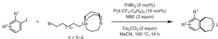
Scheme 1.15 Synthesis of carbocycles using alkyl carbagermatranes.
