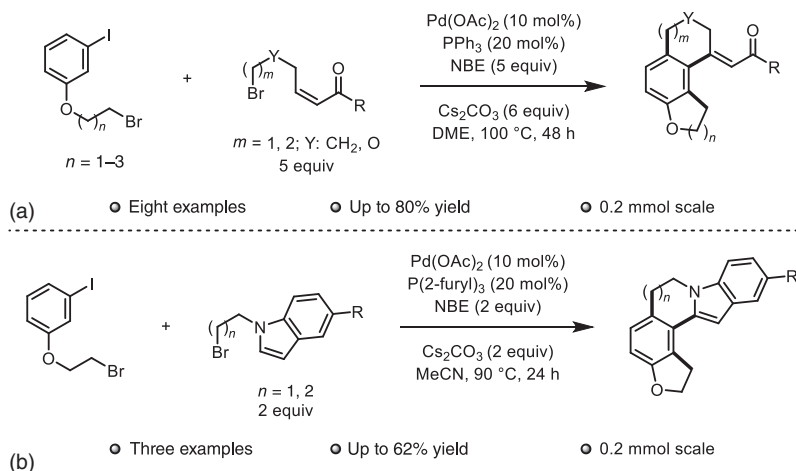
Scheme 1.37 Combining an iodoarene tethered to an electrophile with an electrophile tethered to a terminating group. (a) bromoenoate (b) bromoalkylindole.
