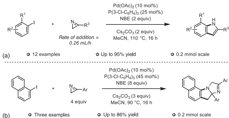
Scheme 1.45 Synthesis of (a) indoles and (b) dihydroimidazoles from aryl iodides and 2 H -azirines.
