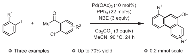
Scheme 1.23 Synthesis of phenanthren-9-ols.
