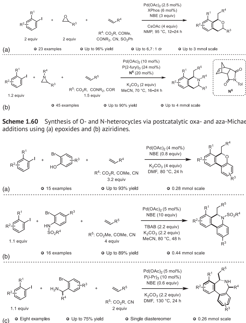
Scheme 1.61 Synthesis of dibenzocycles using (a) ortho -bromophenols, (b) ortho -bromoanilines and (c) ortho -bromobenzylamines.
