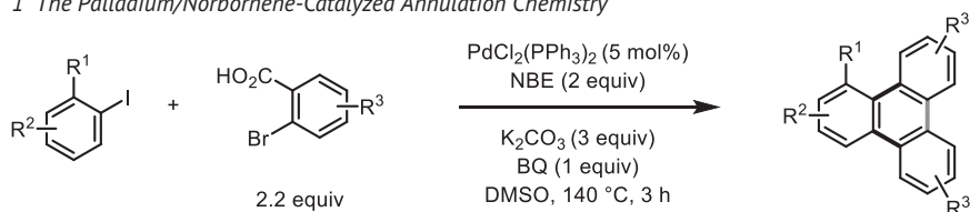
Scheme 1.42 Synthesis of triphenylenes from an aryl iodide and two ortho -bromoarylcarboxylic acids.
