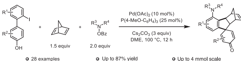
Scheme 1.54 Synthesis of norbornadiene-fused spirocarbocycles via phenol dearomatization.
