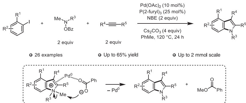
Scheme 1.44 Synthesis of indoles from aryl iodides, O -benzoylhydroxylamines, and alkynes.
