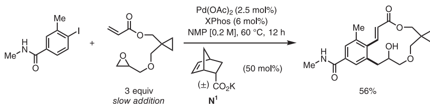
Scheme 1.5 Macrocyclization using an epoxide as an alkylating reagent.
