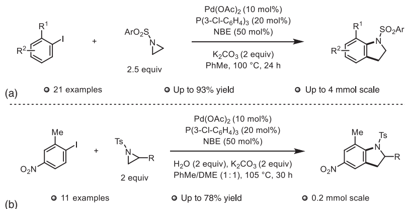
Scheme 1.47 Synthesis of indolines from aryl iodides and (a) 2-unsubstituted aziridines (b) 2-substituted aziridines.
