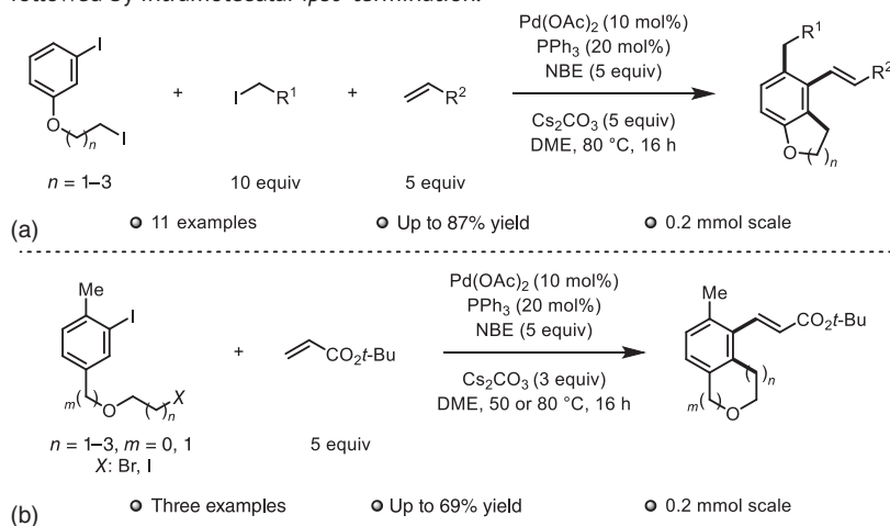
Scheme 1.36 First methodology of ortho -functionalization with a tethered electrophile followed by intermolecular ipso -termination. (a) Unsymmetrical di- ortho -alkylation (b) Mono ortho -alkylation.
