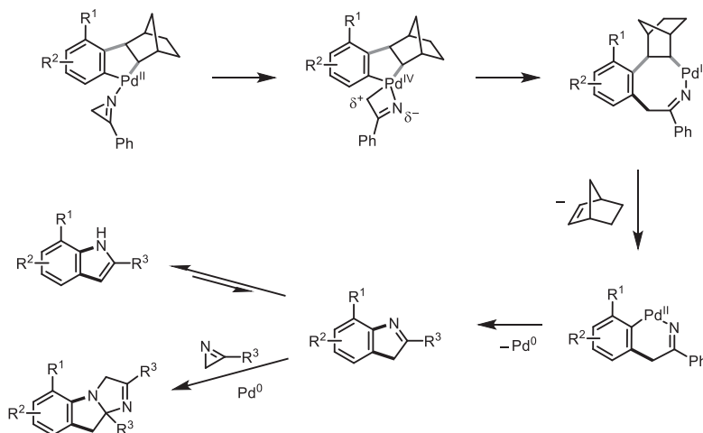
Scheme 1.46 Proposed mechanism for the formation of indoles and dihydroimidazoles from the ANP and 2H-azirine(s).
