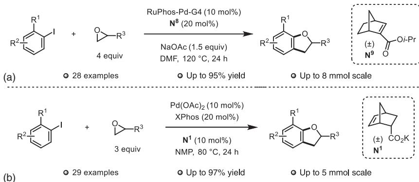
Scheme 1.48 Synthesis of 2,3-dihydrobenzofurans from aryl iodides and epoxides (a) conditions developed by Dong (b) conditions developed by Cheng and Zhou.
