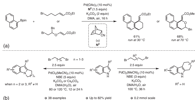
Scheme 1.33 Pd(II)-initiated annulative methodologies using (a) boronic acids and (b) free (N–H) indoles as entry points.
