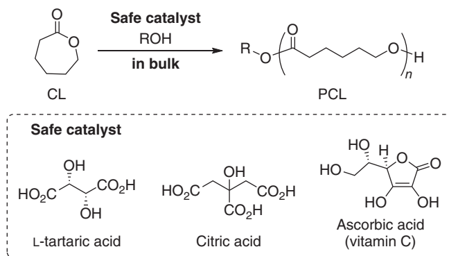
Figure 1.27 ROP of CL and representative truly safe catalysts.
