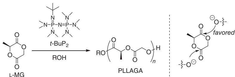
Figure 1.21 Regioselective ROP of MG by the t\text{-BuP}_2 catalyst.
