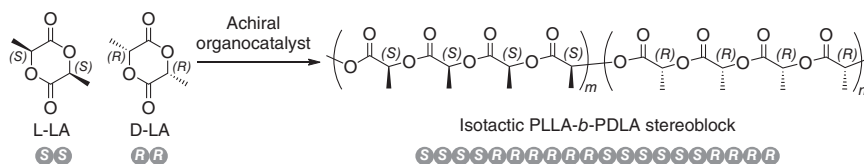
Figure 1.16 ROP of rac -LA using achiral organocatalysts.
