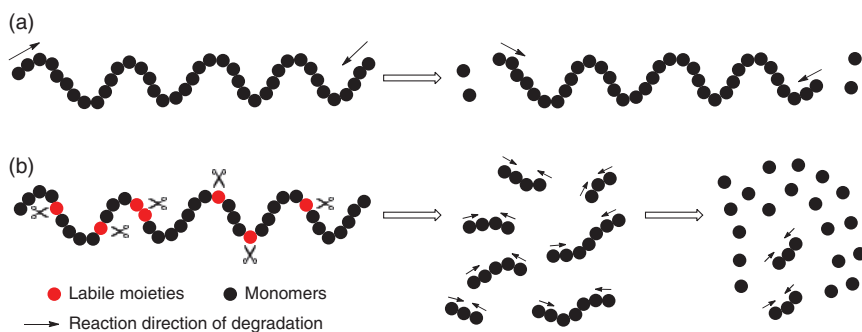
Figure 1.29 Degradation of polymers (a) from the chain ends; (b) from the labile moieties.
