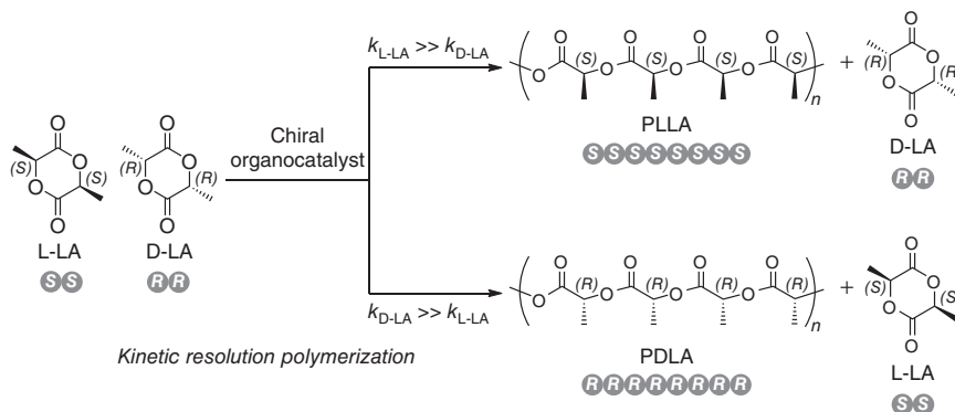
Figure 1.17 ROP of rac -LA using chiral organocatalysts: enantiomer-selective polymerization.
