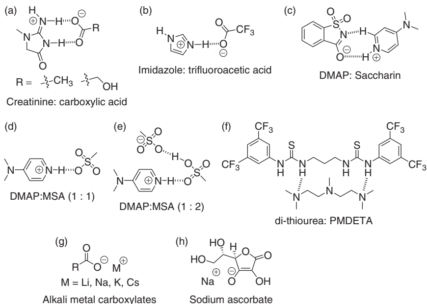
Figure 1.26 Representative acid–base mixed or salt organocatalysts for the ROP of LA in bulk.
