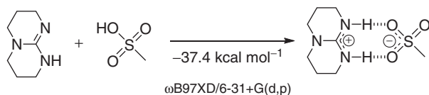
Figure 1.25 Density functional theory calculations of TBD, MSA, and the TBD:MSA (1 : 1) complex.
