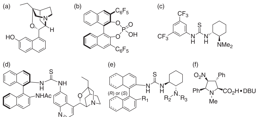
Figure 1.18 Representative chiral organocatalysts for the ROP of rac -LA.
