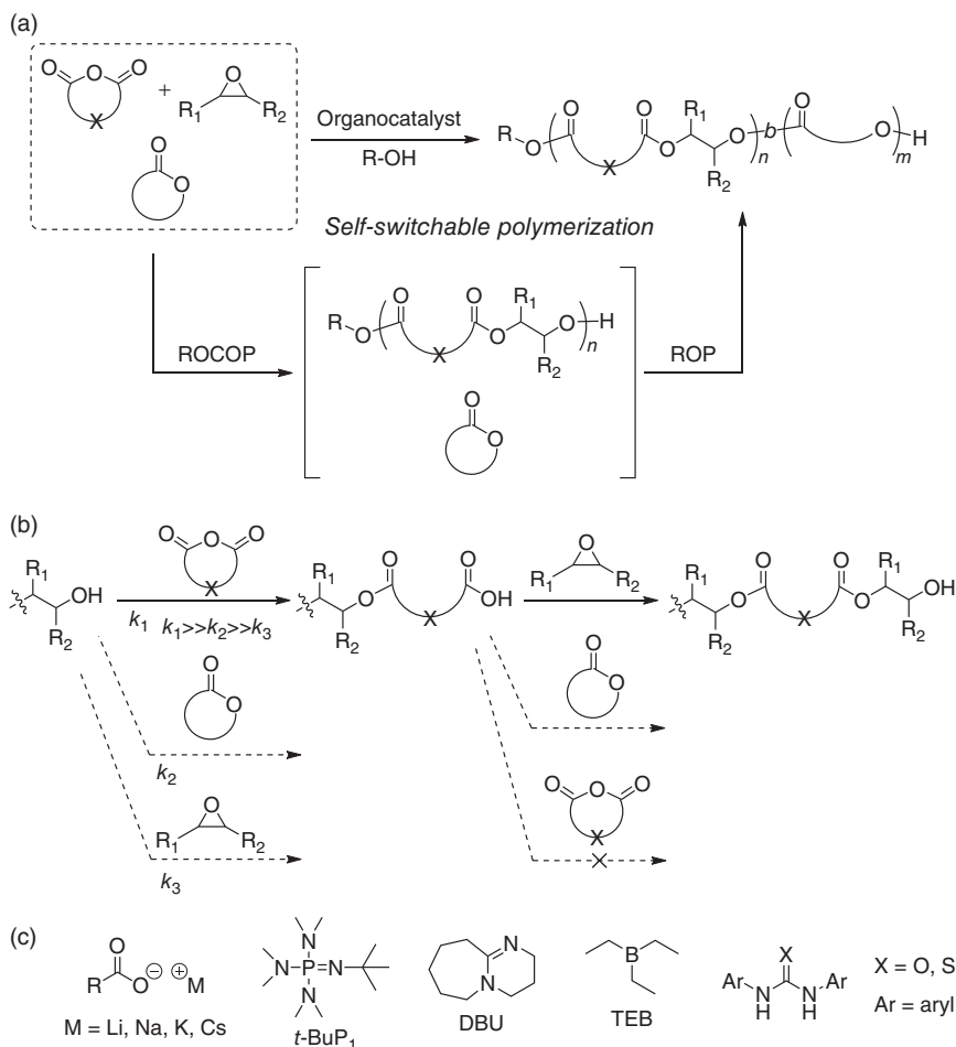
Figure 1.23 (a) Self-switchable polymerization of cyclic anhydrides, epoxides, and cyclic esters; (b) mechanistic consideration of the selectivity; (c) representative organocatalysts.
