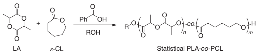
Figure 1.22 Statistical ROP of LA and \epsilon\text{-CL} using a benzoic acid catalyst.
