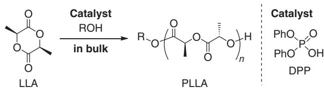
Figure 1.24 ROP of LLA in bulk catalyzed by DPP.
