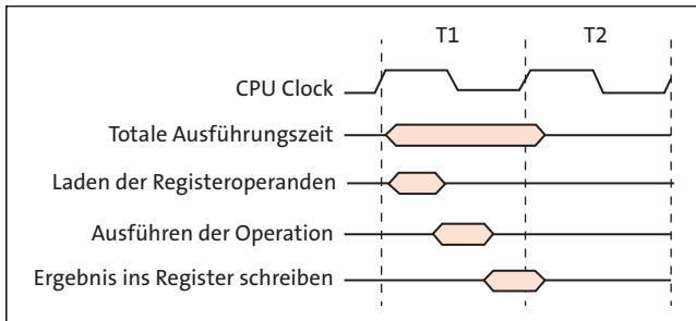
Abbildung 1.8 Single-Cycle-ALU-Operation
