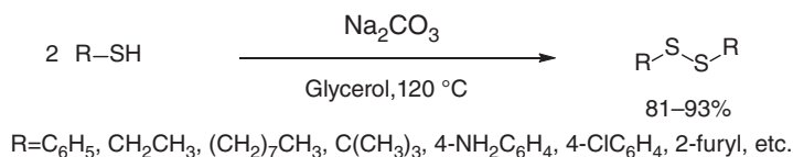
Scheme 1.6 Glycerol as a green solvent in the oxidation of thiols to disulfides.
