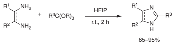
Scheme 1.35 Condensation reaction of benzil, benzaldehyde, and ammonium acetate.
