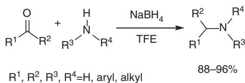
Scheme 1.34 Reductive amination of aldehydes and ketones.
