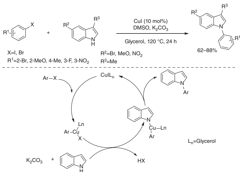
Scheme 1.45 N -arylation of indoles with aryl halides using copper/glycerol.
