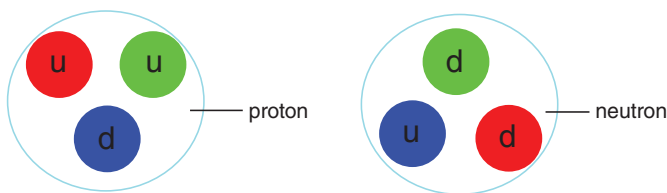
Figure 1.8 Strong interaction among up and down quarks via gluons in protons and neutrons. u: up quark; d: down (or bottom) quark.
