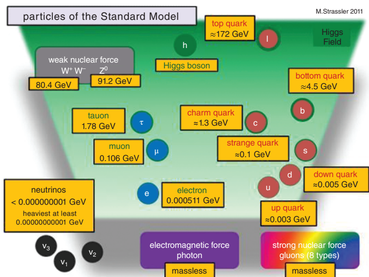
Figure 1.9 Energies or masses of the elementary particles of the Standard Model.
