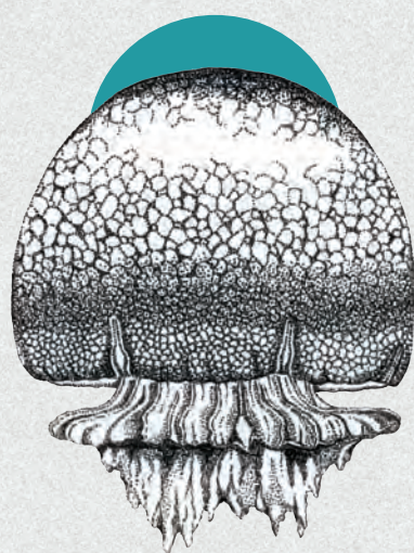
Cannonball Jellyfish
