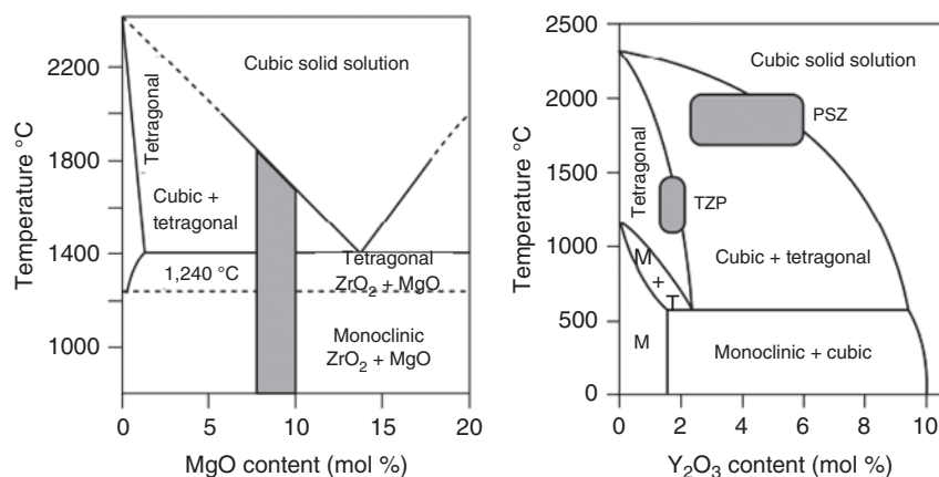
Figure 1.9 Phase diagrams of magnesia (MgO) and yttria ( \text{Y}_2\text{O}_3 )-stabilized zirconia. Source: Hannink et al. [112]/with permission of John Wiley & Sons.
