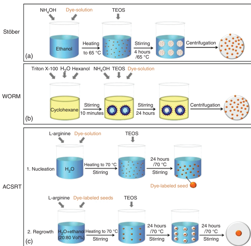
Figure 1.14 Schematic illustration for synthesis of fluorescent silica NPs with three different methods including Stöber (a), water-in-oil reverse microemulsion (WORM) (b), amino acid-catalyzed seed regrowth technique (ACSRT) (c). Source: Shahabi et al. [150]/with permission of Springer Nature.
