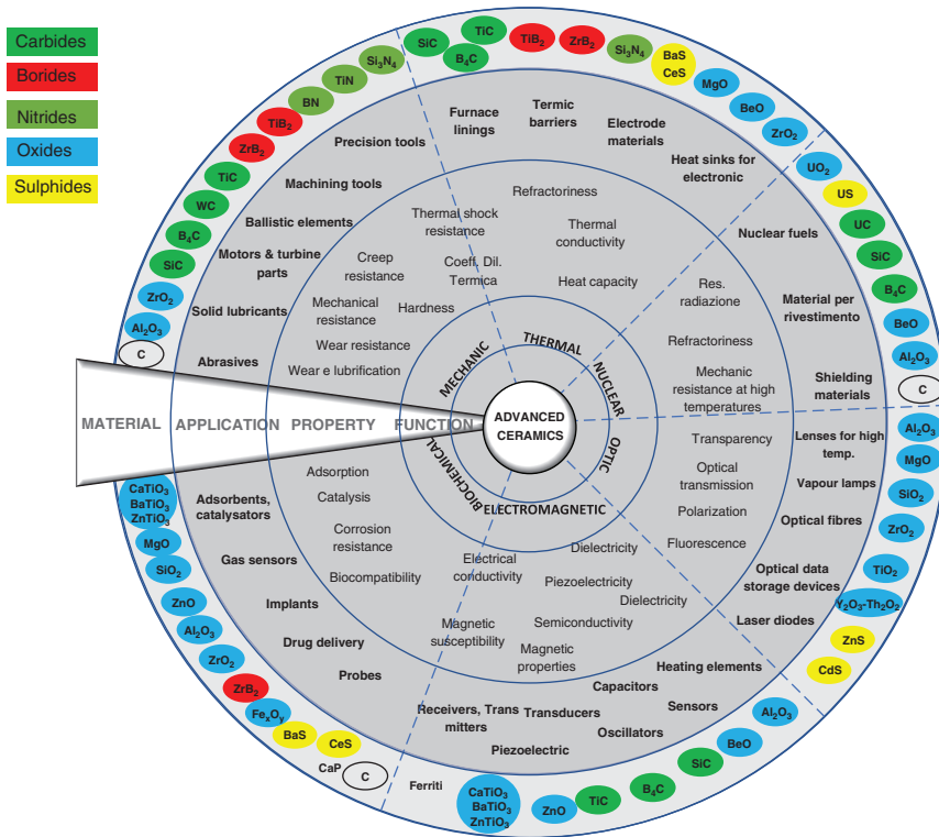
Figure 1.4 Overview of the most relevant advanced ceramics: properties and applications.
