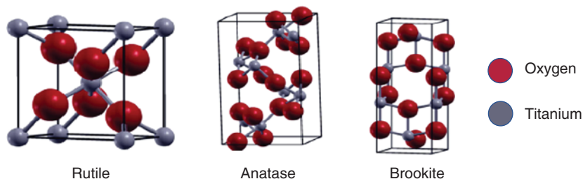
Figure 1.6 Structures of main titania polymorphs (unit cells): rutile, anatase, and brookite. Source: Adapted from Esch et al. [70].
