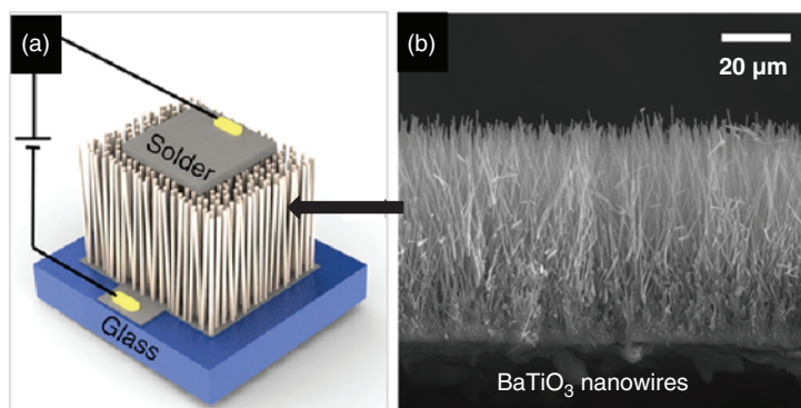
Figure 1.16 (a) Schematic diagram of sensor device using vertically aligned piezoelectric \text{BaTiO}_3 nanowires. (b) A cross-sectional SEM image of \text{BaTiO}_3 NW arrays. Source: Adapted from Koka and Sodano [175]/with permission of Springer Nature.
