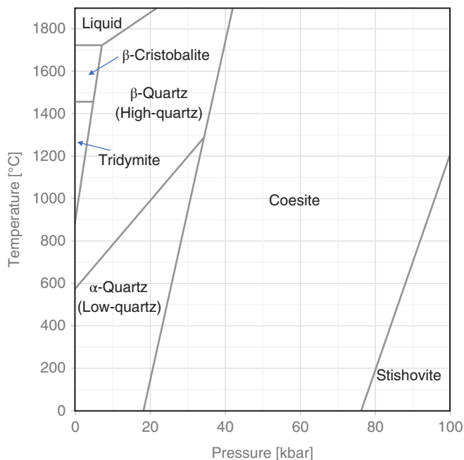
Figure 1.10 Phase diagram for the silica system. Source: Adapted from Lakshitanov et al. [124].
