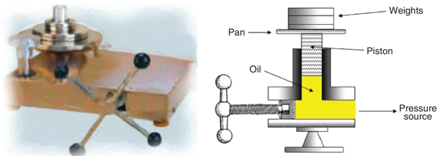
Figure 1.2 Dead-weight gauge.
