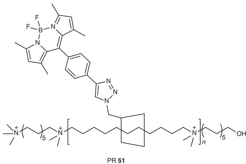
Figure 1.26 Polyrotaxane 51.
