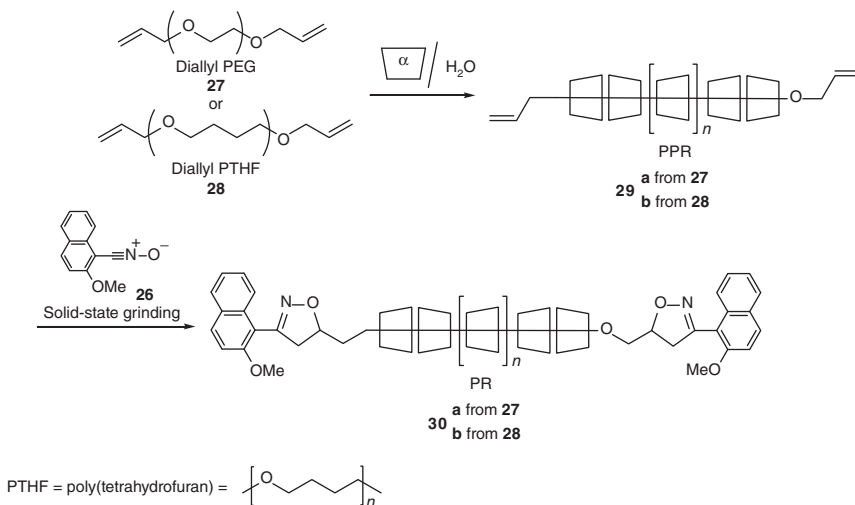
Figure 1.16 Synthesis of polyrotaxanes 30a,b by the sonication followed by solid-state process.
