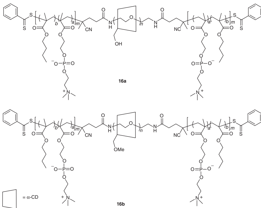
Figure 1.11 Polyrotaxanes 16a,b .
