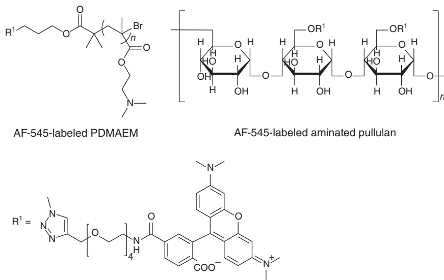
Figure 1.19 The AF-545-labeled PDMAEM and AF-545-labeled aminated pullulan.
