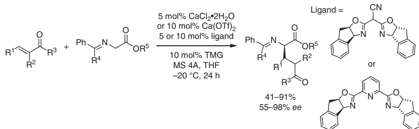
Scheme 1.11 CaCl 2 as the basis of a moisture-tolerant catalytic system.
