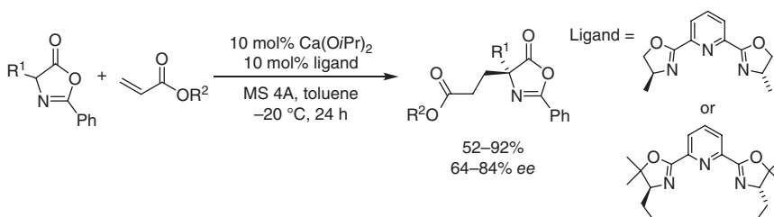
Scheme 1.12 Formation of quaternary stereocenters in the synthesis of glutamic acid derivatives from azlactones.
