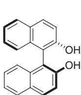
(S)-BINOL
