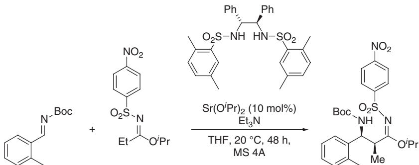
Scheme 1.5 Chiral strontium complex-catalyzed asymmetric Mannich reaction of sulfonylimidates.
