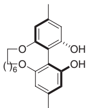
(S)-Biaryldiol
