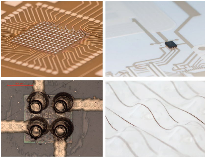
Figure 1.5 Examples of LIFT-printed interconnects and conformal lines on a curved surface.
