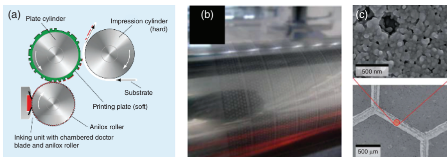
Figure 1.6 Schematic principle of flexo printing (a). (Kipphan (2001) [68]. Reproduced with permission of Springer.) Foil on roll with flexo printed silver ink (b) and microscopic images of the resulting conductive grid structure (c). (Yu et al. (2012) [69]. Reproduced with permission of Royal Society of Chemistry.)
