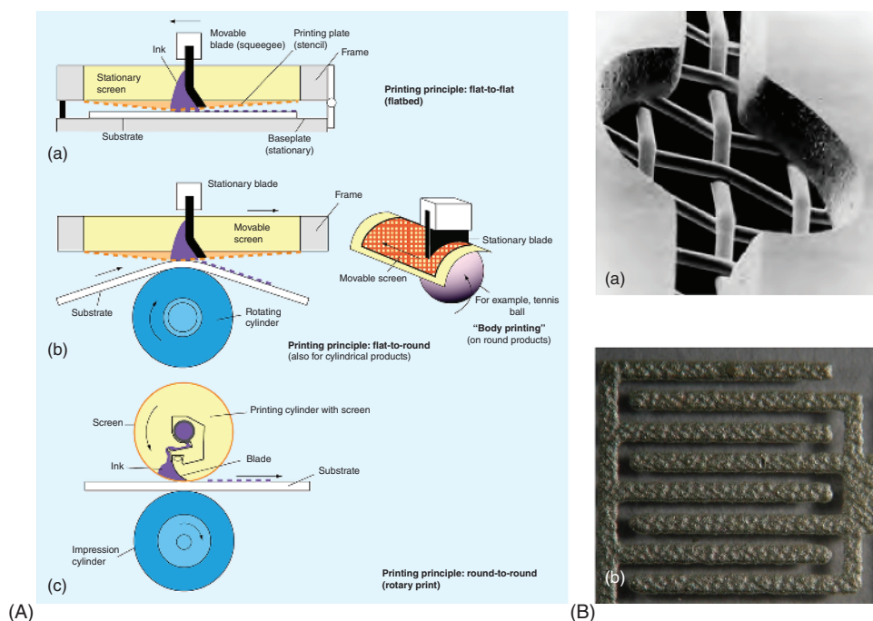
Figure 1.7 Schematic representation of various embodiments of screen printing (A). Electron microscopic image of a screen mesh partially covered with emulsion (B). (Kipphan (2001) [68]. Reproduced with permission of Springer.) Electrode pattern for a pressure sensor consisting of screen-printed graphene sheets and carbon nanotubes [72]. (Janczak (2014) http://www.mdpi.com/1424-8220/14/9/17304/htm . Used under CC BY 3.0 http://creativecommons.org/licenses/by/3.0/ .)
