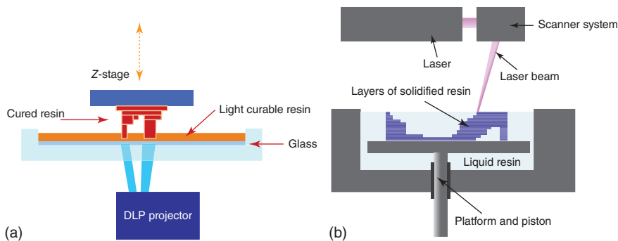
Figure 1.8 Two embodiments of photopolymerization: DLP in which a layer of resin is exposed by a pattern generated by a so-called digital light processor (a) and SLA where the pattern is created by a scanning laser beam (b).
