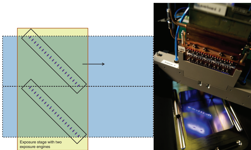
Figure 1.9 Sketch and picture of light engine based on multiple laser sources for high-resolution and large-area 3D printing [82].
