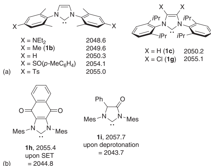
Figure 1.18 (a) Effect of N -aryl and backbone substituents on the TEP values of imidazolylidenes [62, 69]. (b) Examples of switchable NHCs (all values in cm⁻¹).
