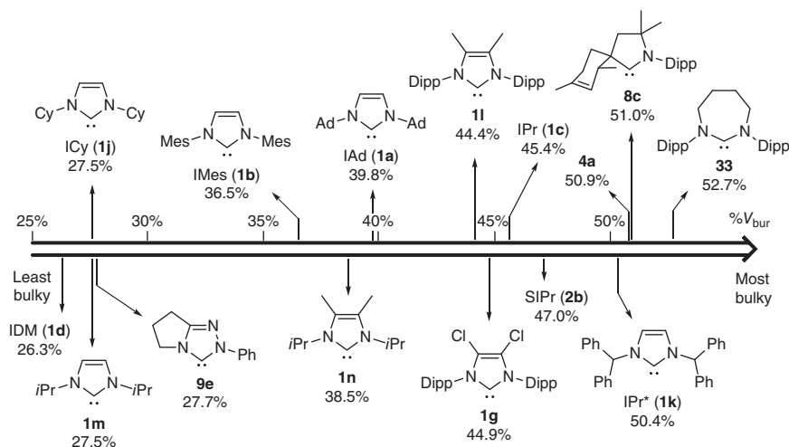
Figure 1.26 Scale showing the variation in \%V_{\text{bur}} values for imidazolylienes with different nitrogen and backbone substituents.
