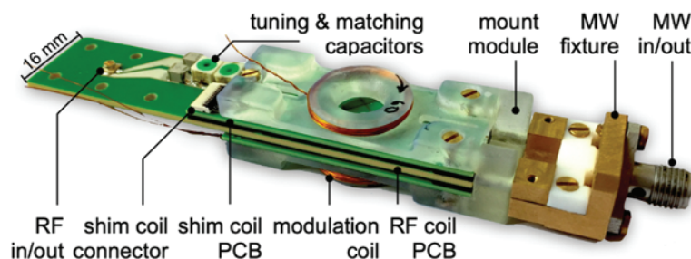
Figure 1.13 Photograph of a fully integrated Overhauser dynamic nuclear polarization (ODNP) probe head, designed to operate in a palm-held 0.5-T permanent magnet. [72] Sebastian Kiss (2019)/figure 05.26 [p.125]/with permission from University of Freiburg.
