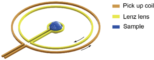
Figure 1.3 The Lenz lens (LL) collects the magnetic flux of the pick-up coil and focuses it into the sample region resulting in an enhanced sensitivity of the measurement.
