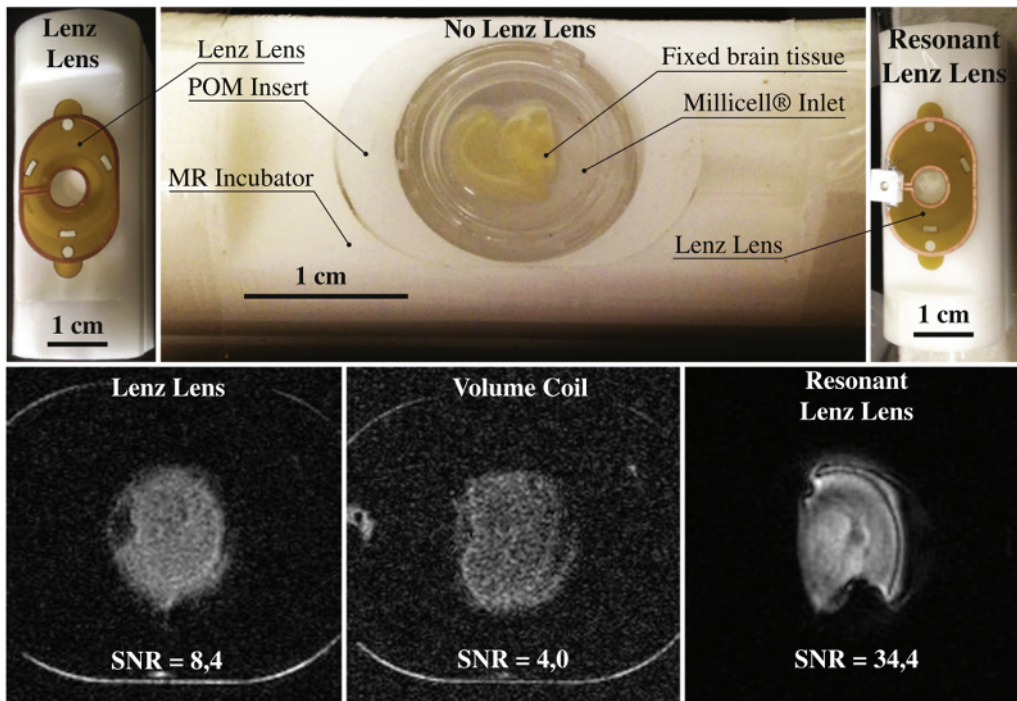
Figure 1.7 Top: Magnetic resonance (MR) compatible incubation platform for cultivating mouse brain slices. The platform was integrated with a broadband nonresonant Lenz lens (LL) (left), and a resonant LL (right). Bottom: MR images of a brain slice using the Bruker volume coil (middle), the broadband LL (left), and the resonant LL (right). [35] R. Kamberger et al. (2018), figure 06[p.13]/with permission from Elsevier.
