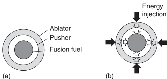
Figure 1.3-15 The principle of inertial confinement fusion. (a) Pellet structure. (b) Implosion and ignition.
