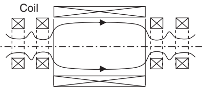
Figure 1.3-2 Tandem mirror.
