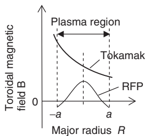
Figure 1.3-11 Magnetic field profile of reversed field pinch.
