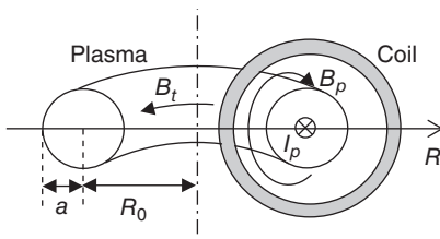
Figure 1.3-8 Tokamak.
