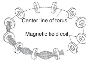
Figure 1.3-14 Configuration of magnetic field coil in bumpy torus. Source: From [11]/Lexington Books.
