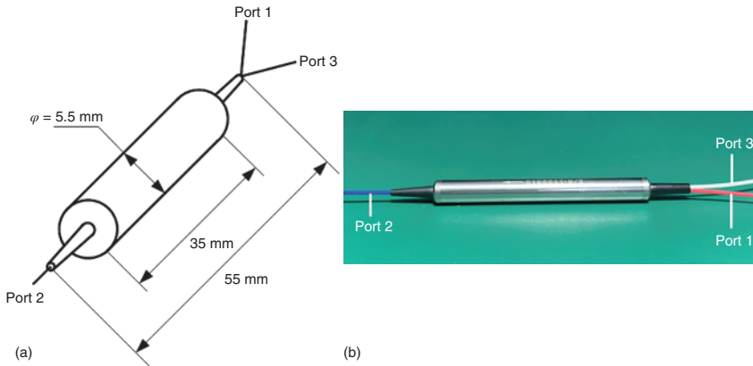
Figure 1.23 (a) Schematic diagram and (b) photo of optical fiber circulator for bidirectional transmission system. Source: Junferg Jiang.
