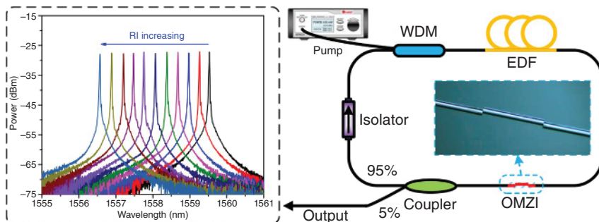
Figure 1.8 Scheme of a tunable fiber ring laser based on OMZI. Source: Junferg Jiang.
