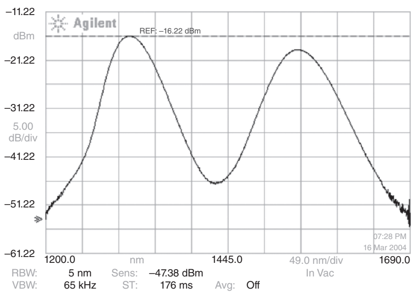
Figure 1.3 Spectrum of a combined SLDs light source. Source: Junferg Jiang.
