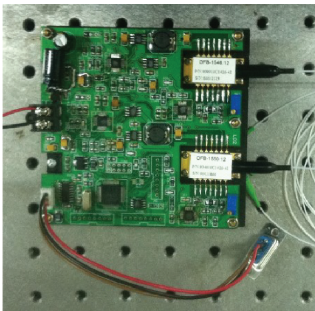
Figure 1.5 Photo of OEM light source with two pigtailed DFB lasers. Source: Junferg Jiang.
