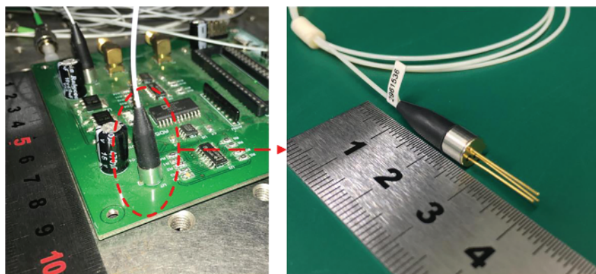
Figure 1.16 TO can pigtailed photodiode and its use in a demodulation circuit. Source: Junferg Jiang.
