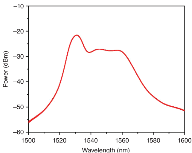
Figure 1.7 Typical ASE spectrum of an EDF. Source: Junferg Jiang.
