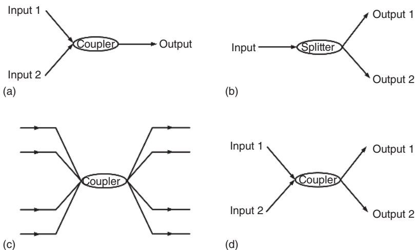
Figure 1.17 Coupler port configuration. (a) Y-coupler (b) optical fiber splitter (c) star coupler (d) X-coupler. Source: Junferg Jiang.
