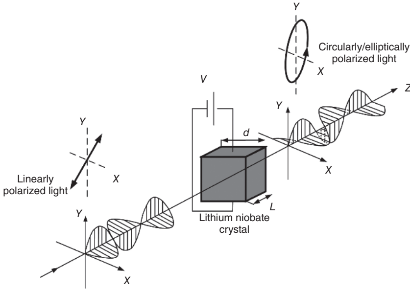
Figure 1.28 Schematic of electro-optical fiber modulator based on lithium niobate. Source: Junferg Jiang.
