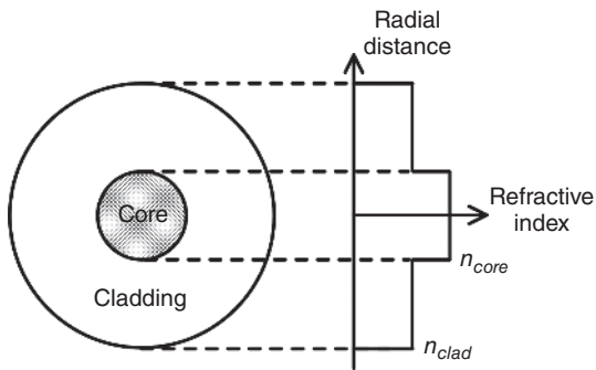
Figure 1.1 Cross-section refractive index profile of typical optical fiber. Source: Junferg Jiang.
