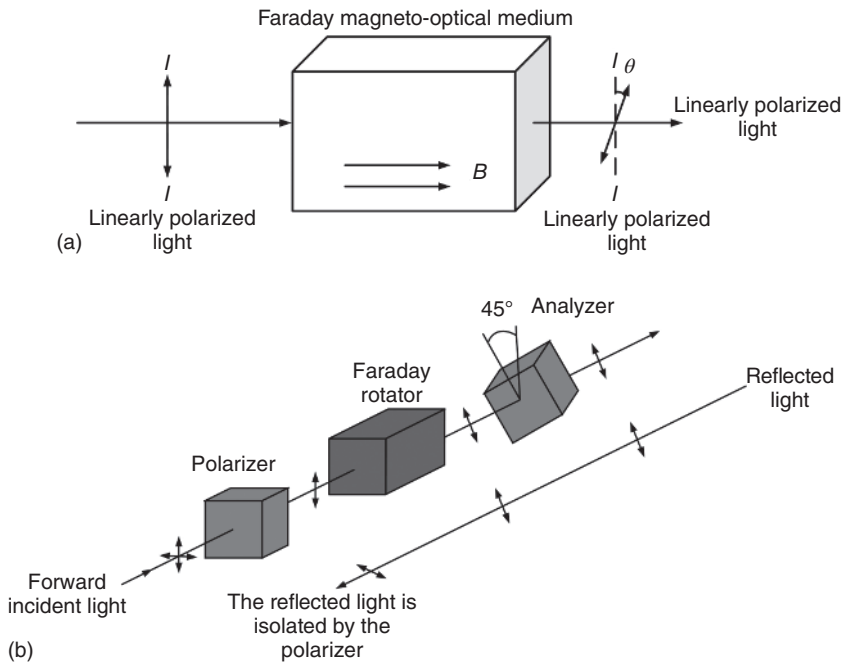
Figure 1.19 Schematic diagram of (a) Faraday magneto-optical effect and (b) optical fiber polarization dependent isolator. Source: Junferg Jiang.
