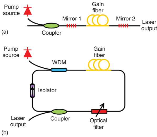
Figure 1.6 Schematic diagrams of the optical fiber lasers with (a) linear cavity and (b) ring cavity. Source: Junferg Jiang.
