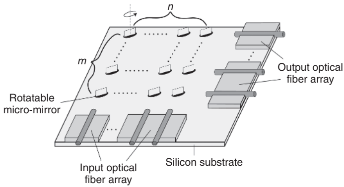
Figure 1.25 MEMS m \times n optical fiber switcher matrix. Source: Junferg Jiang.
