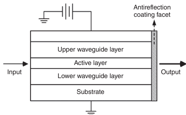
Figure 1.13 Schematic diagram of SOA. Source: Junferg Jiang.
