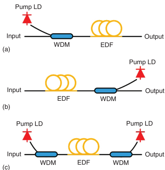
Figure 1.11 Schematic diagrams of EDFA with three optical pumping methods: (a) forward pump, (b) backward pump, and (c) dual-directional pump. Source: Junferg Jiang.
