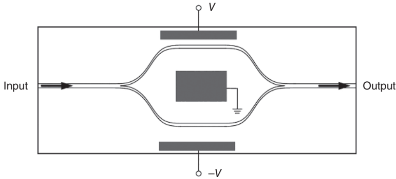
Figure 1.29 MZI optical fiber intensity modulator. Source: Junferg Jiang.
