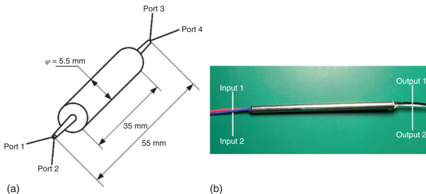
Figure 1.18 (a) Schematic diagram and (b) photo of 2 \times 2 optical fiber coupler. Source: Junferg Jiang.
