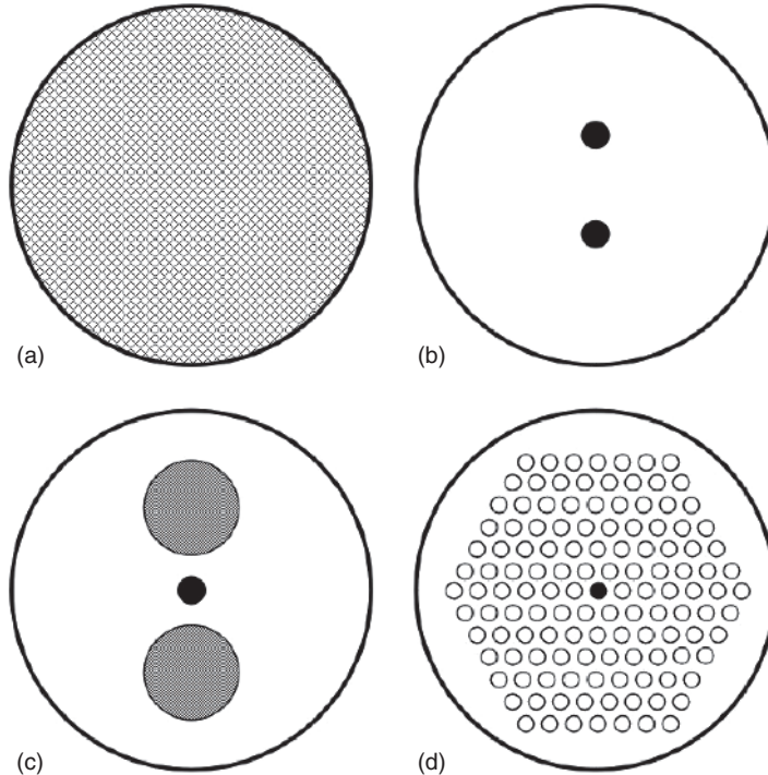
Figure 1.2 Scheme of special optical fibers: (a) NCF, (b) TCF, (c) PMF, and (d) PCF. Source: Junferg Jiang.
