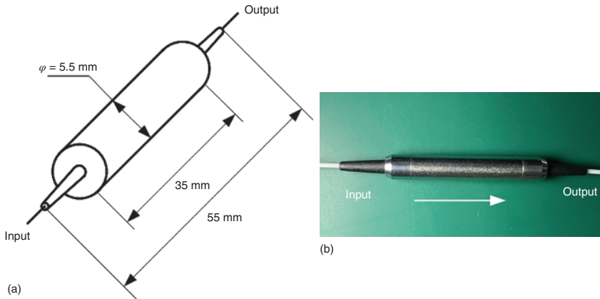
Figure 1.21 (a) Schematic diagram and (b) photo of 2 \times 2 optical fiber isolator. Source: Junferg Jiang.
