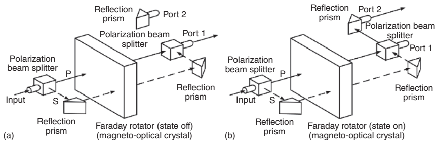
Figure 1.27 Schematic of 1 × 2 magneto-optical fiber switcher. (a) Optical path from input to port 1. (b) Optical path from input to port 2. Source: Junferg Jiang.
