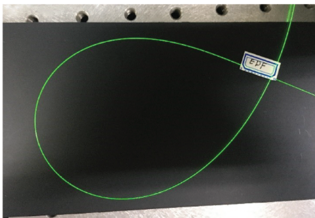
Figure 1.9 Green fluorescence of EDF pumped by 980 nm light. Source: Junferg Jiang.
