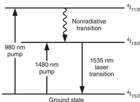
Figure 1.10 The pertinent energy diagram of \text{Er}^{3+} . Source: Junferg Jiang.
