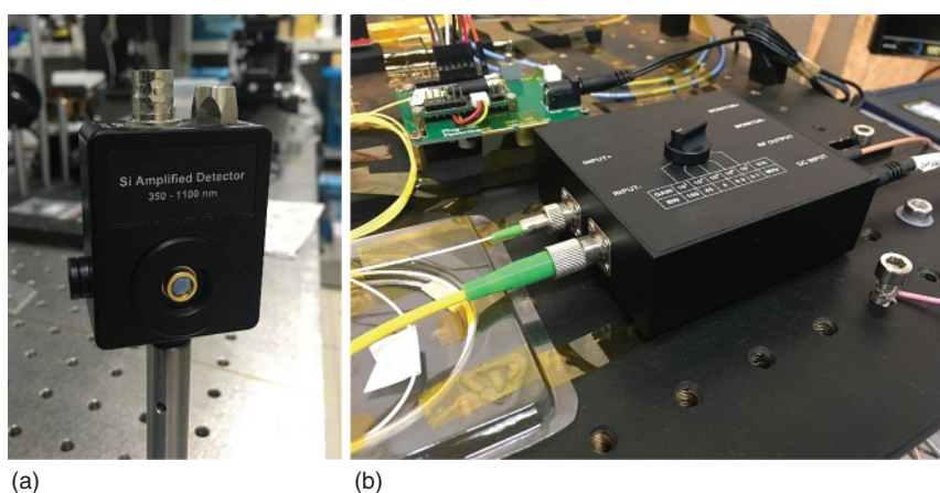
Figure 1.15 Photos of (a) a Si-amplified photodetector with space coupling input and (b) a balanced photodetector with two fiber inputs. Source: Junferg Jiang.
