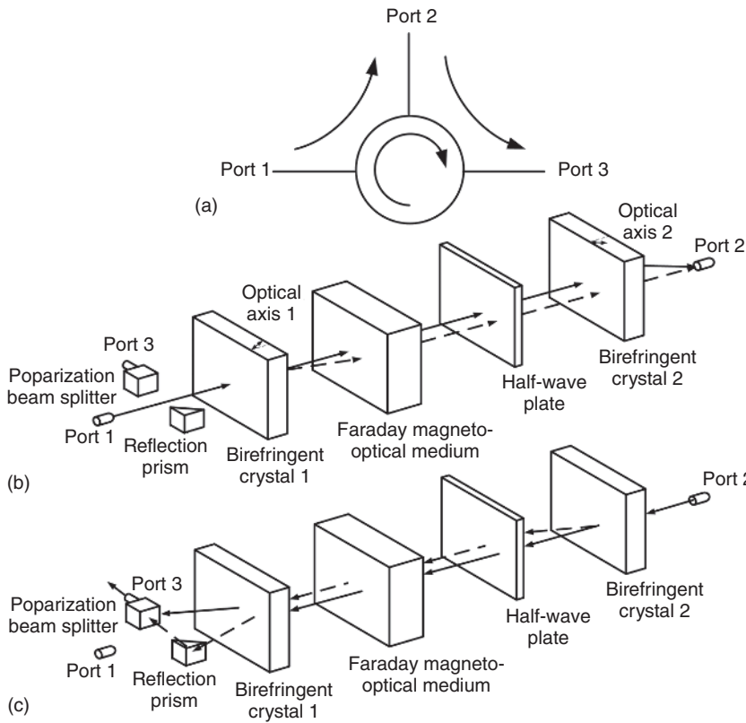
Figure 1.22 (a) Schematic of three-port optical fiber circulator, (b) optical path from port 1 to port 2, and (c) optical path from port 2 to port 3. Source: Junferg Jiang.
