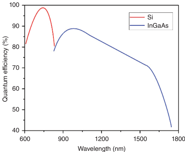
Figure 1.14 Wavelength responses of Si- and InGaAs-based photodiodes. Source: Junferg Jiang.
