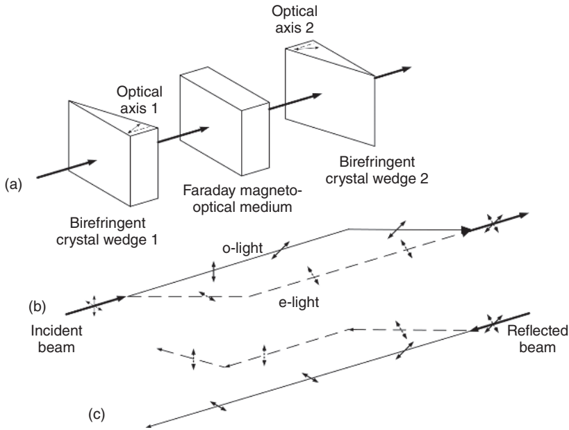
Figure 1.20 (a) Schematic diagram of optical fiber polarization-independent isolator. Light path of (b) incident light and (c) reflected path (top view). Source: Junferg Jiang.
