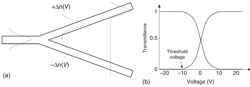
Figure 1.26 Electro-optical fiber switcher (a) structure and (b) numerical characteristics [16]. Source: Modified from Silberberg et al. [16].
