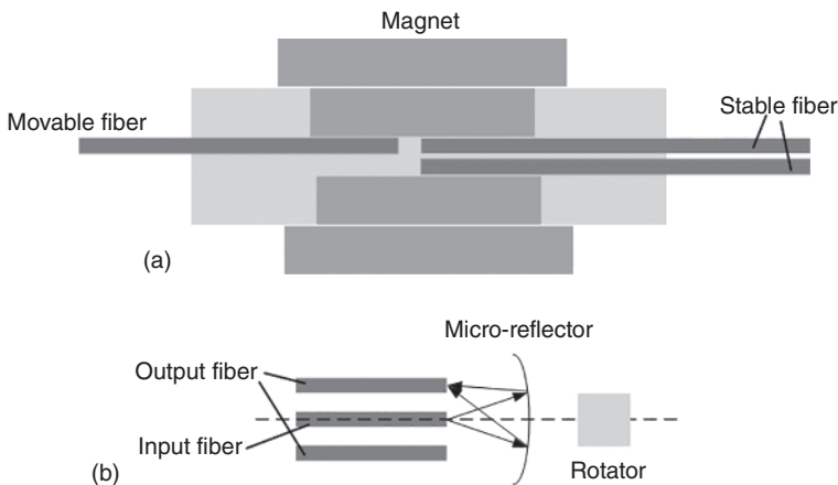
Figure 1.24 Mechanical optical fiber switchers based on (a) magnet and (b) reflector. Source: Junferg Jiang.
